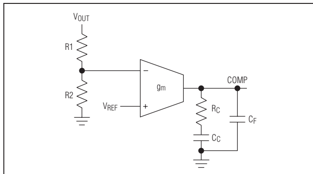
Figure 4. Compensation Network
